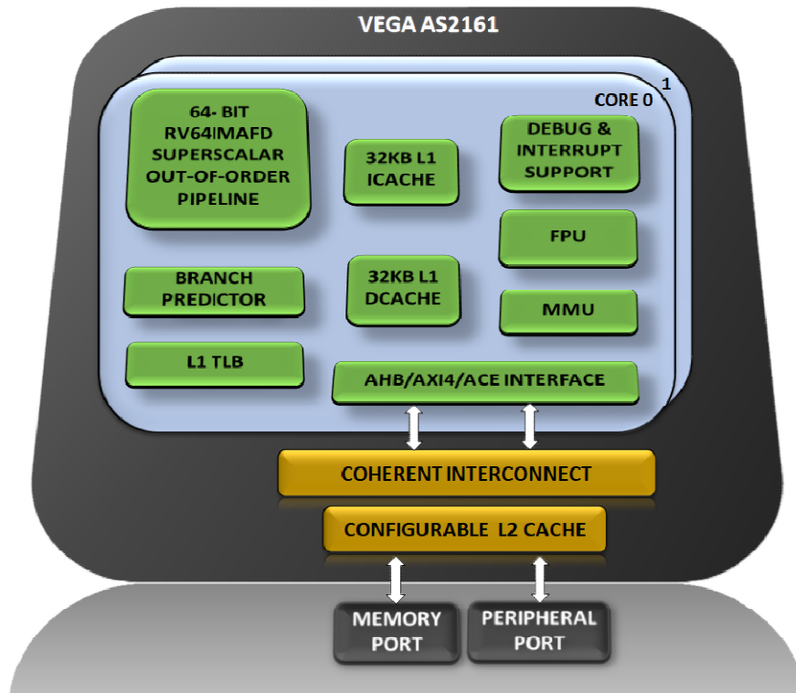
Figure 1: VEGA AS2161 Block Diagram
